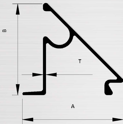
Glazing Clip
