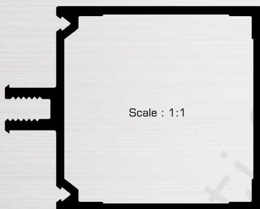
Curtain Wall
