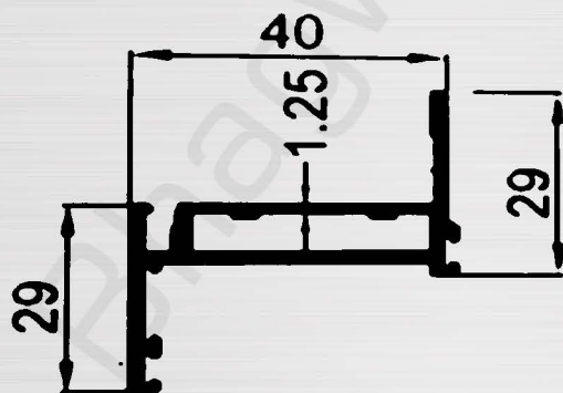
Z Hollow (40 Series)
