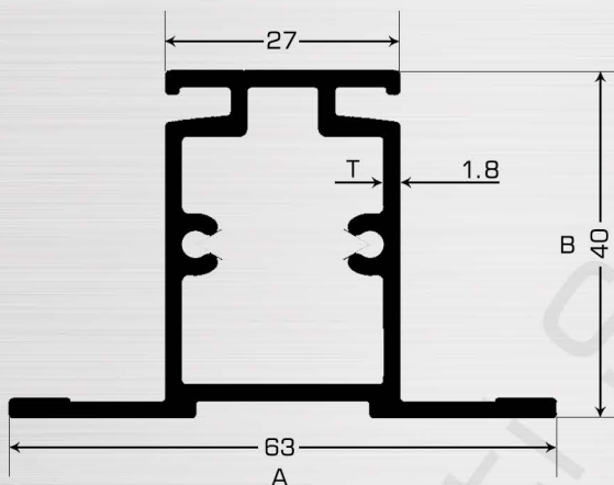
Mullion (40 Series)
