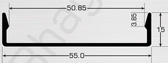
Cover Plate
